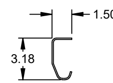
3" Track (Opt.) .105 Galv. Steel (12 ga.)
