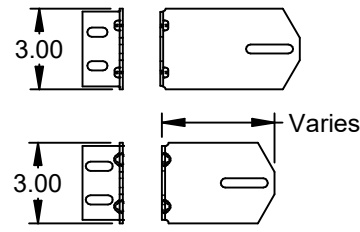
Track Bracket .116 Galv. Steel (11 ga.)
