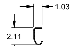
2" Track .055 Galv. Steel (16 ga.)
