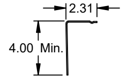
2" Angle Mount (Opt.) .086 Galv. Steel (13 ga.)
