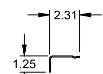
2" Clip Angle (Opt.) .086 Galv. Steel (13 ga.)
