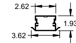
Center Stile .063 Extruded Aluminum
