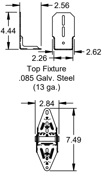
Top Fixture .085 Galv. Steel (13 ga.)
