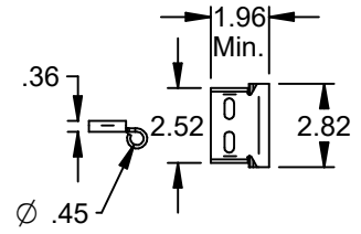
Roller Carrier .114 Galv. Steel (11 ga.)
