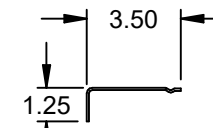
3" Clip Angle (Opt.) .086 Galv. Steel (13 ga.)
